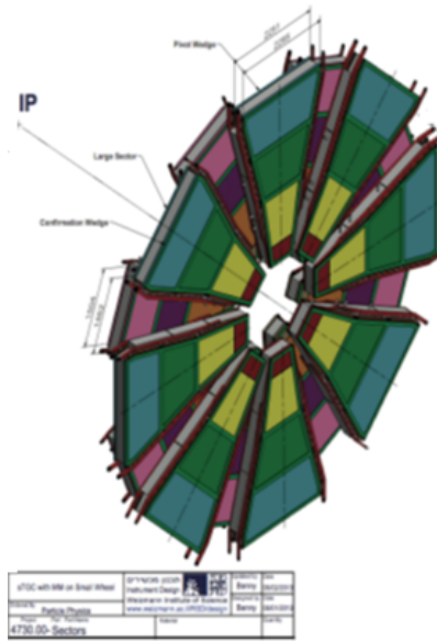
Figure 5.20: The new Small Wheel Layout.
