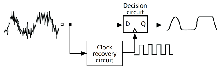
Figure 2.7: The role of a CDR circuit in retiming data.
