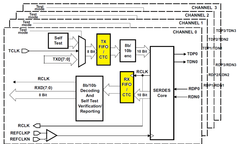
Figure 2.25: Block Diagram of LK3134 SerDes for XAUI1000BaseX applications.
