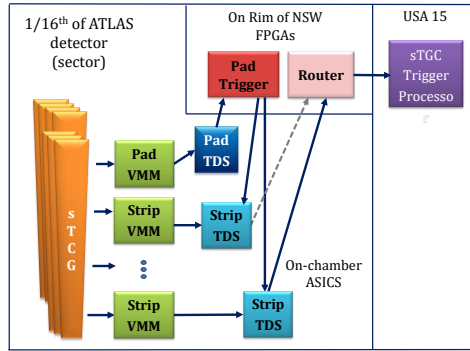
Figure 5.26: The sTGC trigger scheme.
