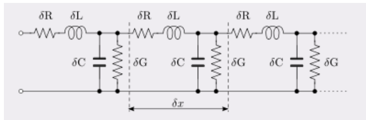
Figure 2.5: Equivalent circuit diagram of a transmission cable.
