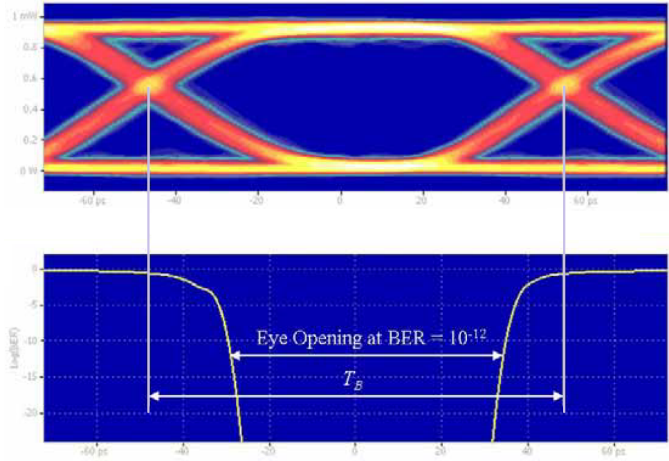
Figure 2.16: An eye diagram (top) and the corresponding bathtub-plot: The bit error ratio as a function of the time-position of the sampling point with respect to the ideal logic transition time, BER(x) .
