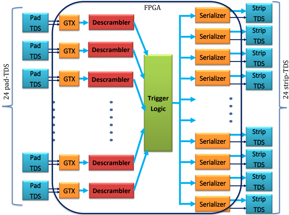
Figure 5.27: FPGA-pad trigger internal structure.
