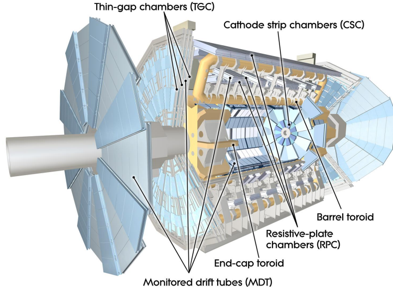
Figure 4.10: The ATLAS Muon Spectrometer.
