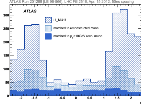
Figure 5.19: \eta distribution of L1 trigger signal coming from muons with p_T > 10 \text{ GeVc}^{-1} (L1_MU11) with the distribution of the subset signal coming from muon candidates which match (within \Delta R < 0.2 ) to offline well reconstructed muons (combined inner detector and muon spectrometer track with p_T > 3 \text{ GeVc}^{-1} ), and offline reconstructed muons with p_T > 10 \text{ GeVc}^{-1} .
