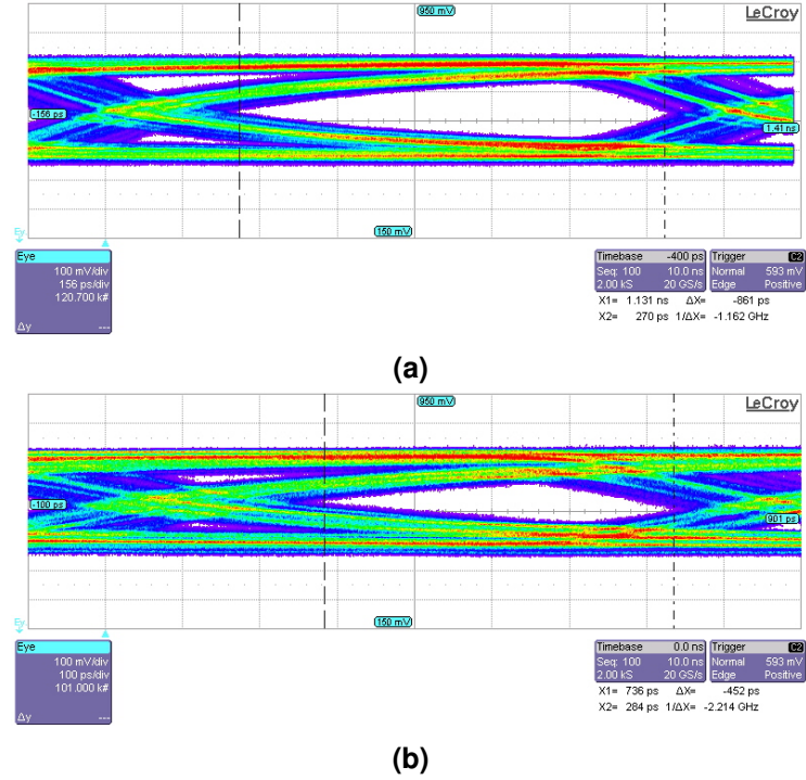
Figure 5.35: The Eye Diagram obtained sending on a 4 m miniSAS cable a pseudo random pattern at 800 Mbps (a) and 1250 Mbps (b) .
