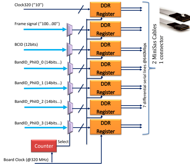
Figure 5.33: Output logic to the strip-TDS .
