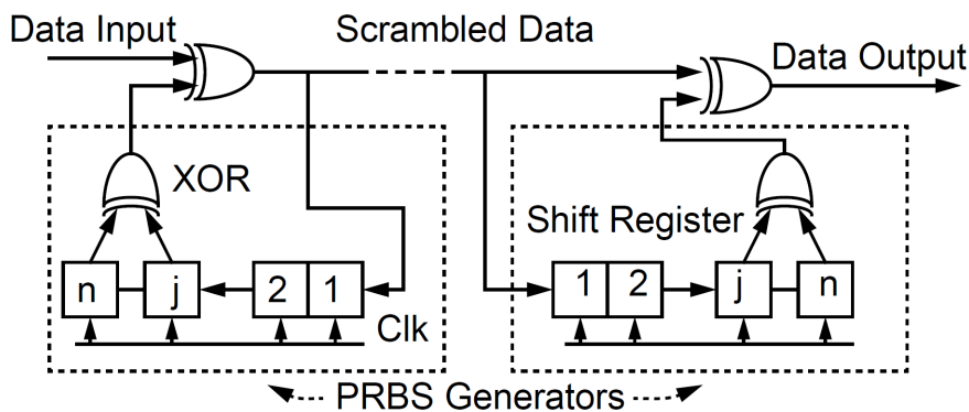
Figure 2.4: Scrambling. A feedback shift register is used to randomize data and in order to restore original data another register, which reverses the process, is used at receiver.
