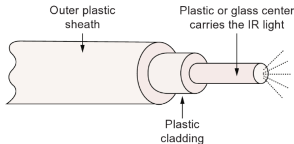
Figure 2.6: Structure of a an optical fiber cable.
