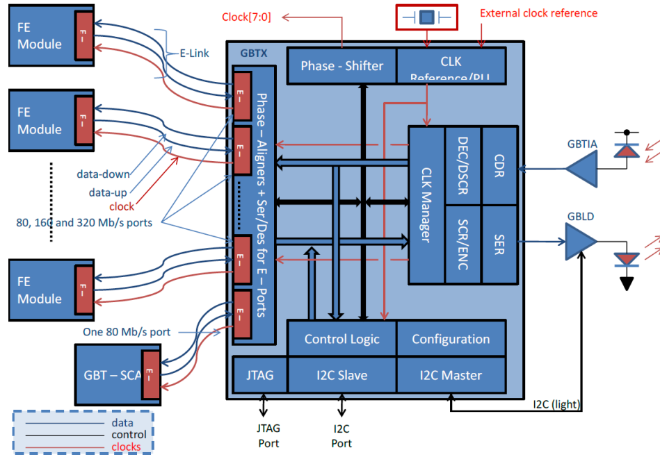
Figure 2.21: A simplified block diagram of the GBTx.
