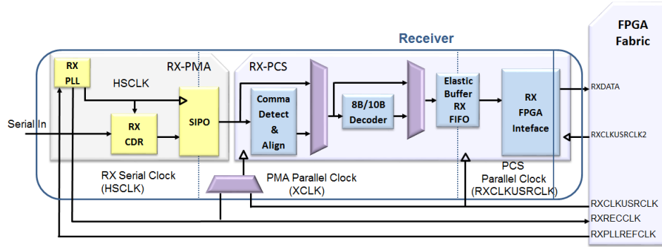
Figure 5.28: Receiver section of the GTX transceiver.
