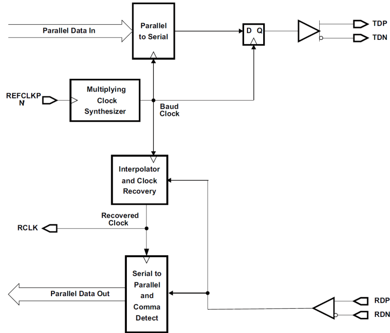
Figure 2.24: Core Block Diagram of the TLK3134 SerDes.
