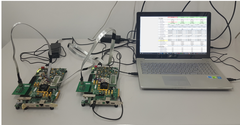
Figure 5.36: Set up for testing the transmission quality of the miniSAS cable.
