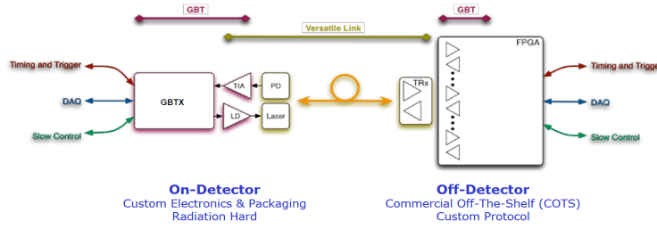
Figure 2.20: Radiation-hard optical link architecture.
