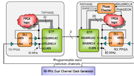
Figure 5.31: Fixed latency link.
