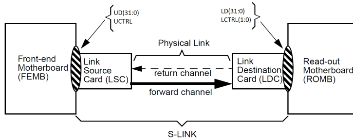
Figure 2.19: S-LINK Concept and data format.
