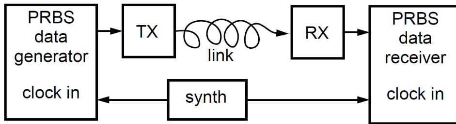
Figure 2.13: Typical BER Test set-up.
