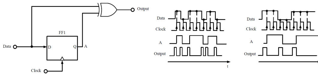
Figure 2.9: Basic linear phase detector (left) and output waveforms (right).
