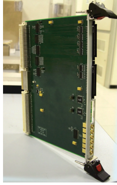
Figure 5.6: Current MUCTPI Interface board.
