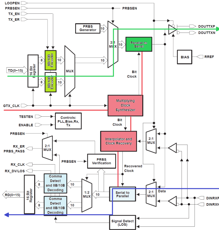
Figure 2.23: TLK1501 Block Diagram.
