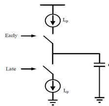
Figure 2.11: Charge pump in PLL.
