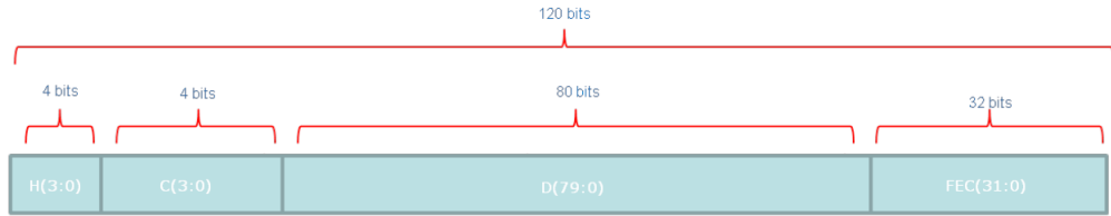
Figure 2.22: GBT frame format.
