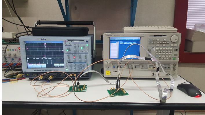
Figure 5.34: Set up for testing the transmission quality of the miniSAS cable.
