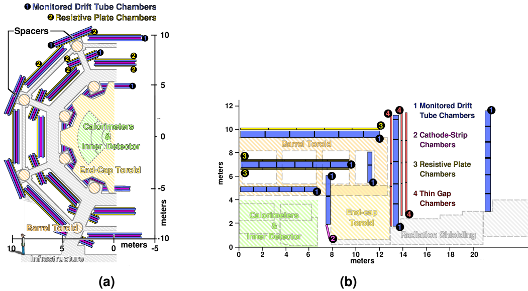
Figure 4.11: The cross-section of the barrel muon system perpendicular to the beam axis showing three concentric cylindrical layers (a). The cross-section of the muon system in a plane containing the beam axis (b).
