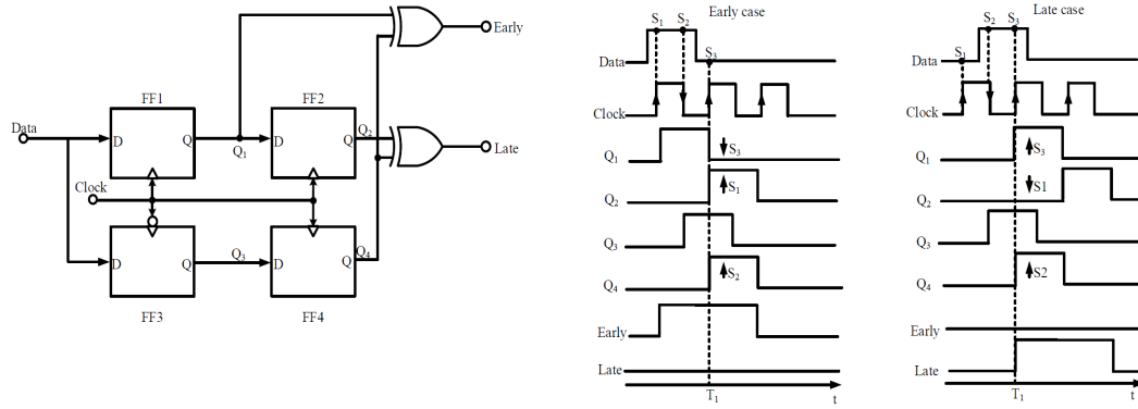
Figure 2.10: Alexander Linear phase detector.
