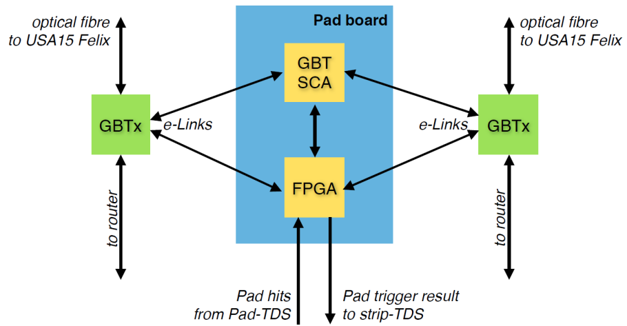
Figure 5.39: Pad trigger board to GBT connections.
