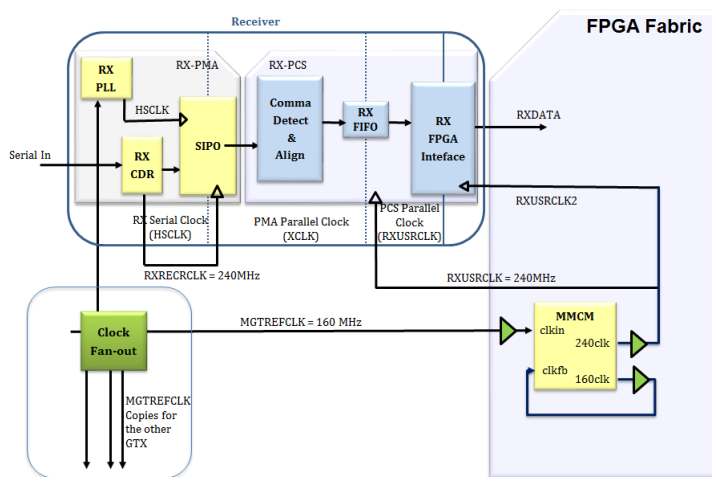
Figure 5.30: Fixed latency receiver architecture.
