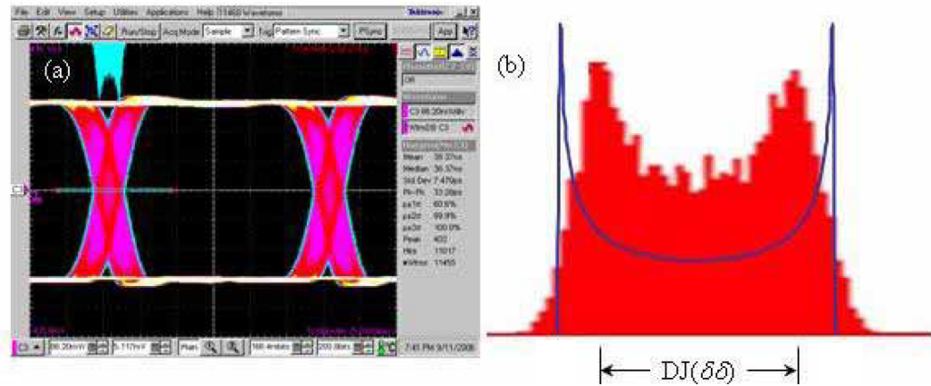
Figure 2.15: An eye diagram (left) and the corresponding TJ histogram (right).
