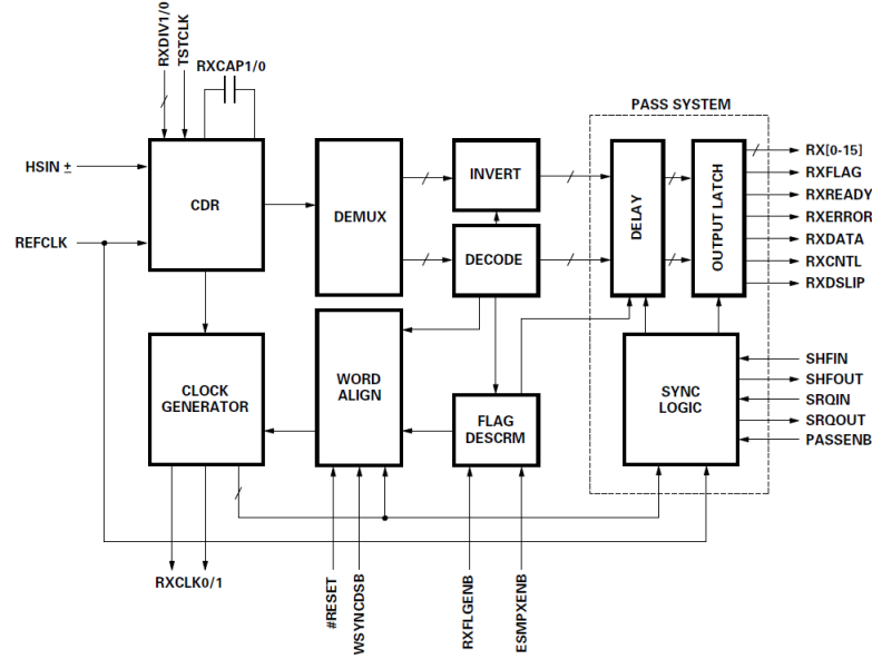
Figure 2.18: Block Scheme of the Receiver chip in G-Link.
