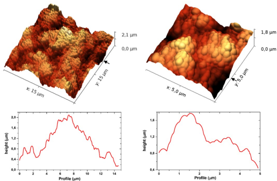
Fig. 5.18. AFM micrographs of a slide glass covered by JWSPs (top-left) and a magnification (top-right), with height profiles (bottom), corresponding to the arrows.
