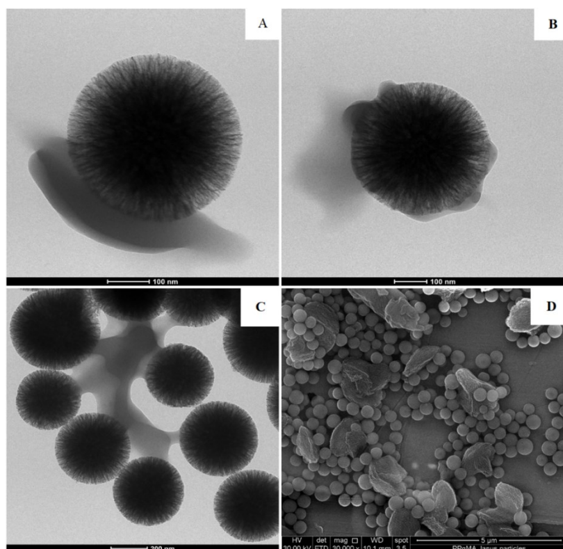
Fig. 5.25. TEM micrographs showing the Janus character of PPgMA grafted wrinkled particles (A, B) and TEM and SEM images showing clusters formation (C, D).
