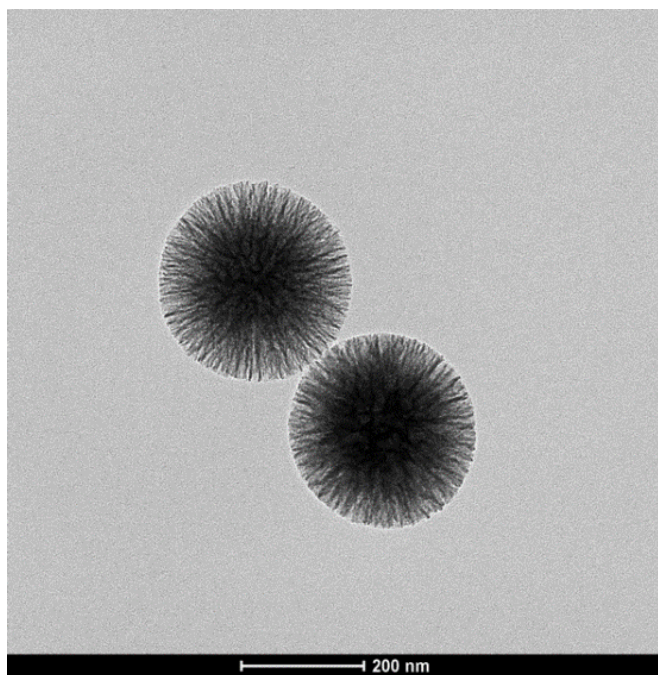
Fig. 5.14. Wrinkled and clean structure of JWSPs.
