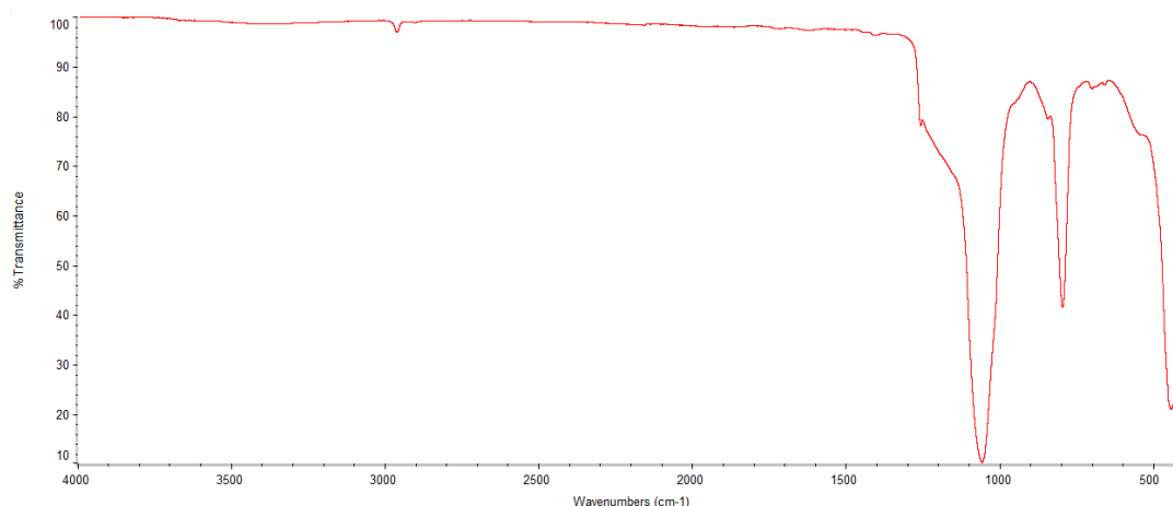
Fig. 5.16. ATR spectrum of JWSPs powder characterized by a short pick at 2965 \text{cm}^{-1} due to the \text{CH}_3 asymmetric stretching vibration.
