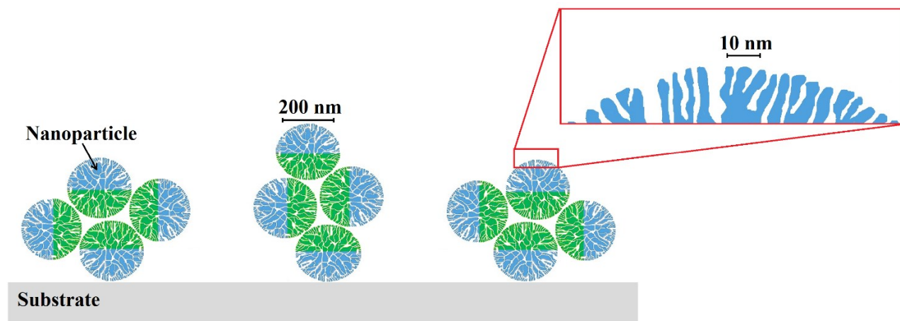
Fig. 1.7. Hierarchical structure formed by deposition of cluster of JWSPs, blue and green zones are characterized by different chemical physical behaviour. the multilevel hierarchy is on micron level for clusters, hundreds of nanometer for particles size and nanometers for the wrinkles of the silica-gel particles.
