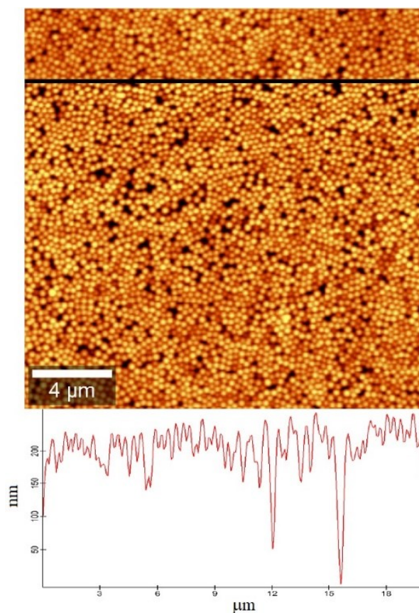
Fig. 5.19. AFM micrographs of a slide glass covered by wrinkled particles (top) and a height profiles (bottom), corresponding to black line in the top figure.
