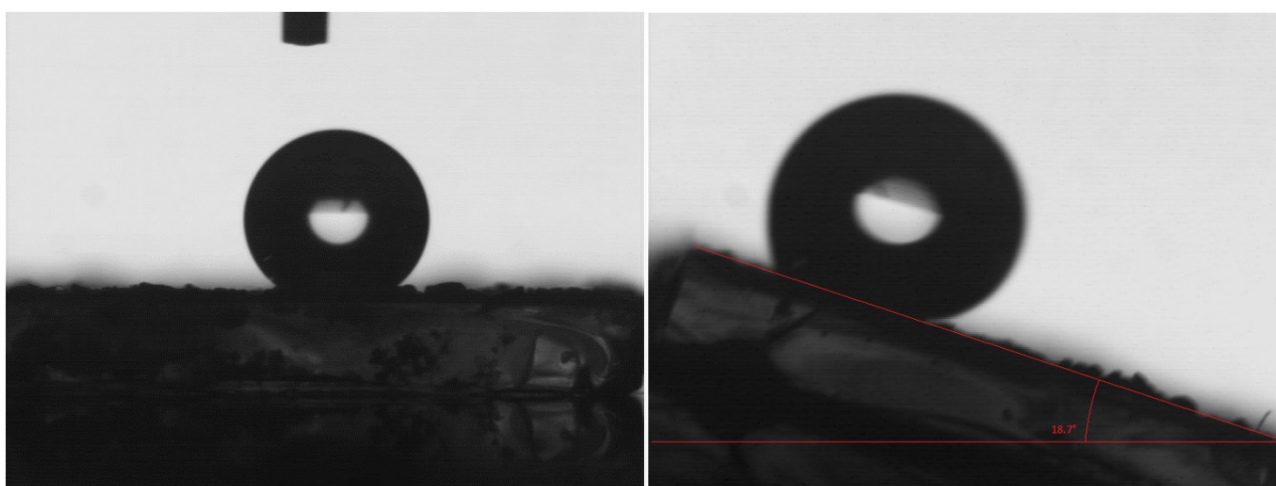
Fig. 5.21. Droplet of water on horizontal surface coated with smooth Janus particles (left) and droplet during rolling off from the inclined coated substrate (right).
