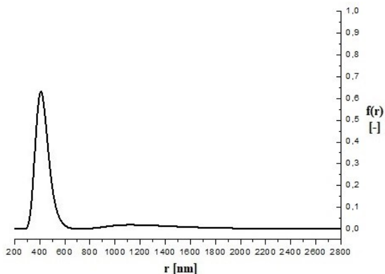
Fig. 5.17. Distribution of the radius, in nanometers, of the JWSPs as determined by DLS.
