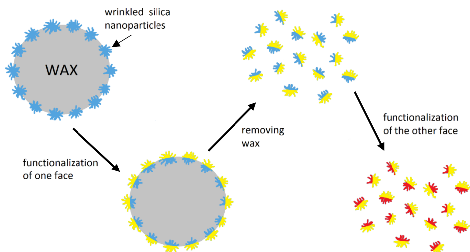
Fig. 1.8. Pathway for the production of JWSPs. The first step involves the surface functionalization on wax for production of hydrophilic-hydrophobic JWSPs (blue and yellow particles). The grafting of the polymer chains involves the last step of the process, forming polymer grafted JWSPs (red and yellow particles).
