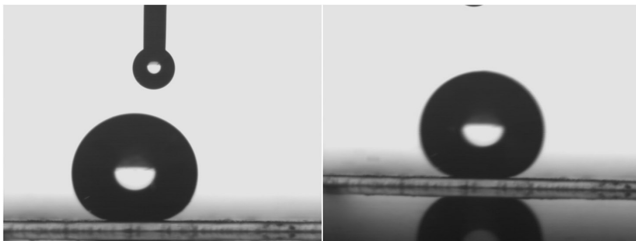
Fig. 5.22. Droplet of water on horizontal surface coated with JWSPs (left) and droplet during rolling off from the inclined coated substrate (right).
