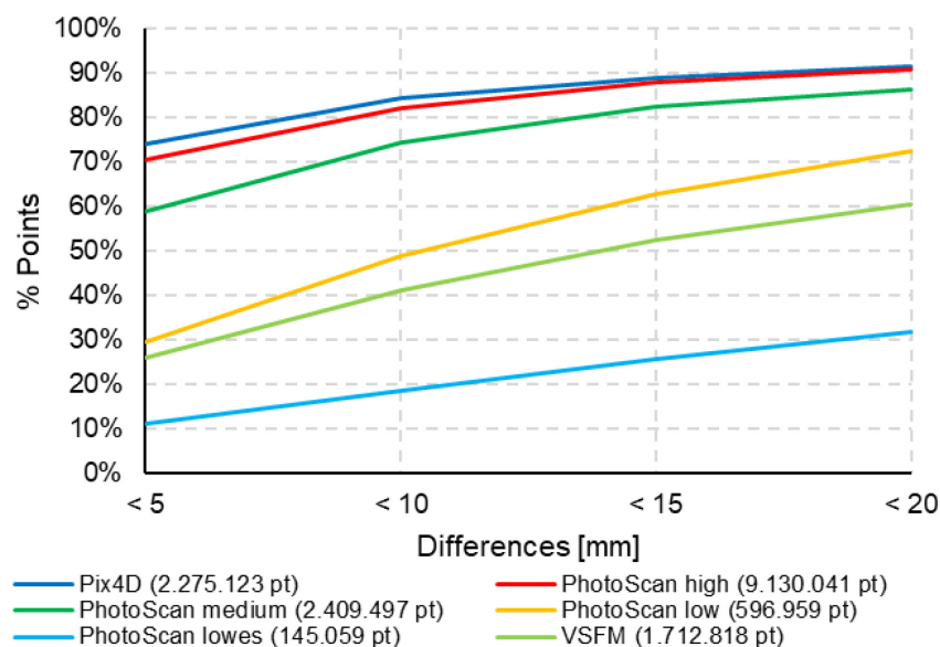
Figure 3.19: Statistics of the differences between BLK 360 scans and the different SFM-Models
