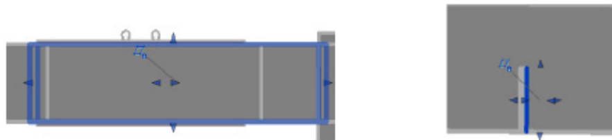
Figure 4.2: Modelling the passing (left) and not-passing (right) cracks in a BIM environment.
