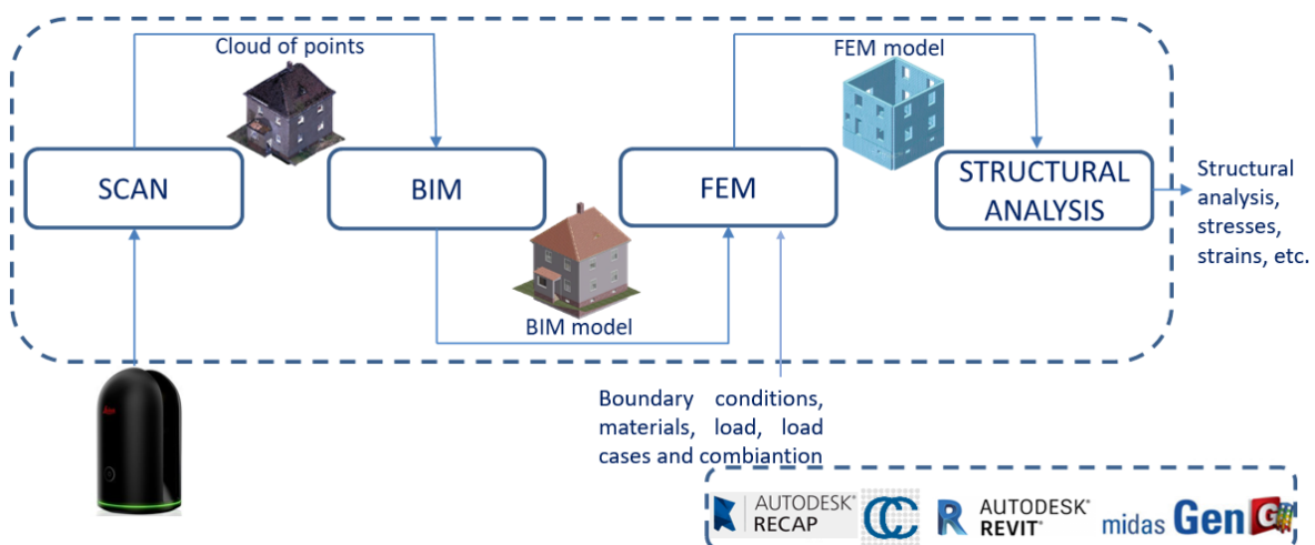
Figure 3.21: Scan-to-FEM process
