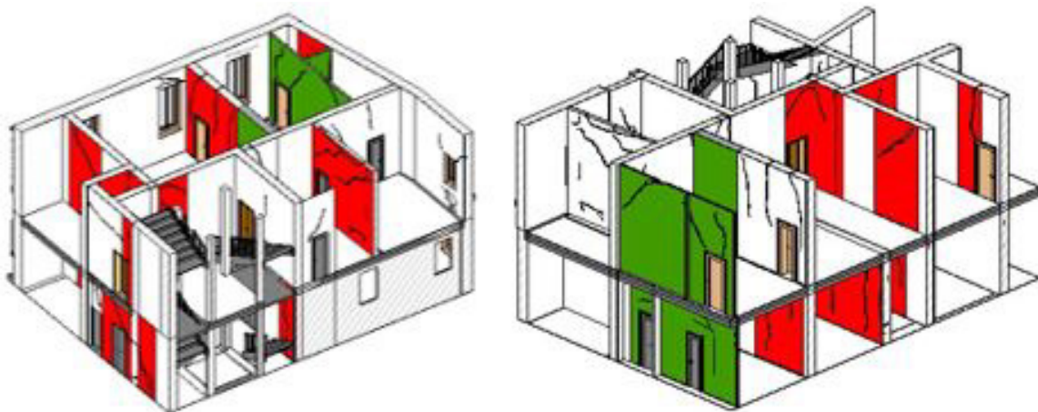
Figure 4.13: Views of the BIM model of the building, with the passing and non-passing cracks highlighted.
