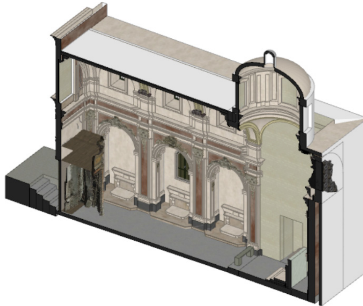
Figure 6.21: Axonometric views and cutaways of the architectural BIM model realized by the DiARC team
