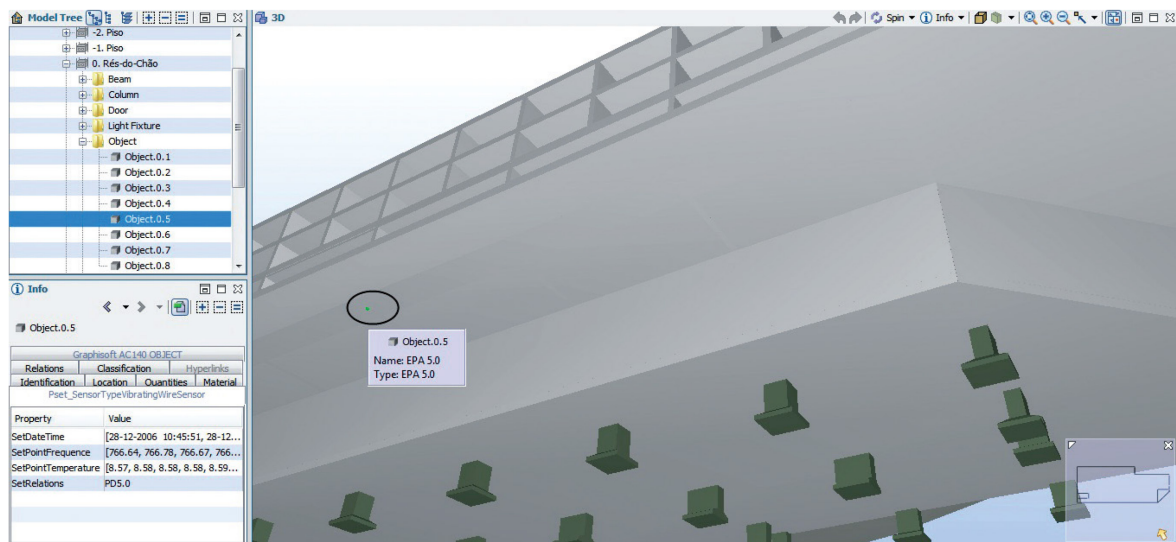
Figure 1.34: BIM model of a bridge provided with sensors [36]
