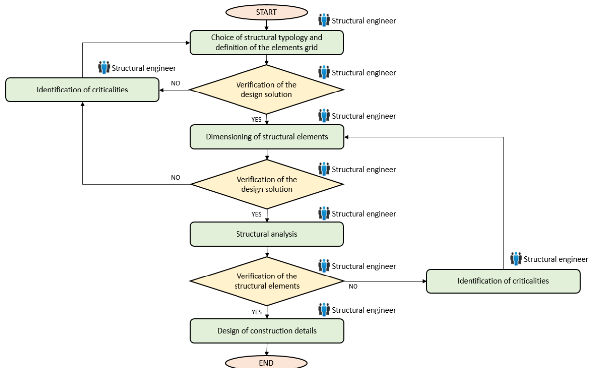
Figure 1.39: Example of workflow for the structural design
