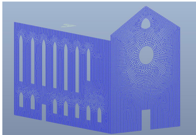
Figure 3.49: FEM model of the Santa Chiara monastery's façades
