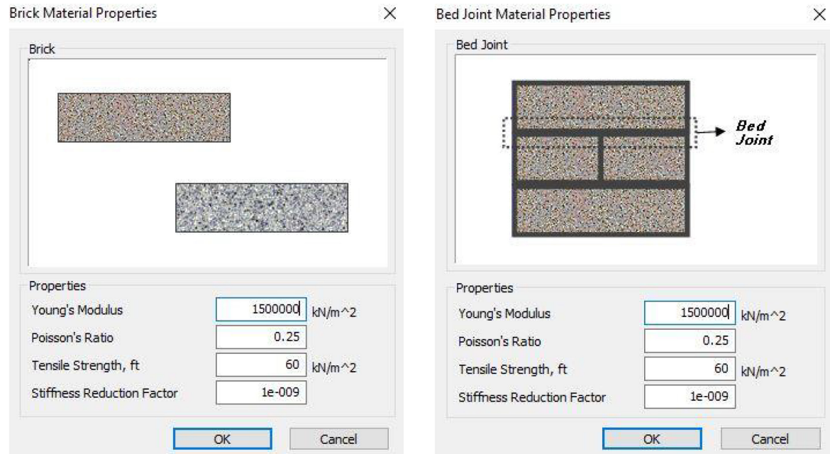
Figure 3.32: Mechanical parameters of masonry material according to Strumas Model.
