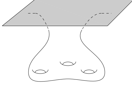
FIGURE 1.1: An asymptotically flat manifold with just one end. By the definition, such manifolds can possibly have a quite complicate topology but all “concentrated” in a bounded domain.
