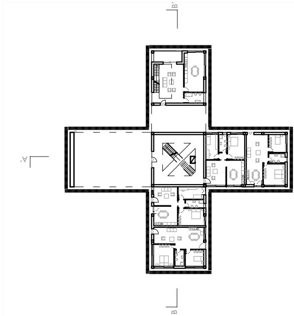
PIANTA PIANO TERRA +1.20
