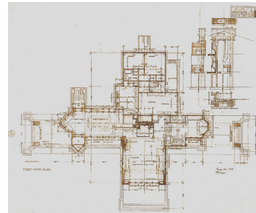
F. L. WRIGHT, WARD W. WILLITS HOUSE, HIGHLAND PARK (ILLINOIS), 1902. PIANTA PIANO PRIMO. DA: PFEIFFER, B. B. GOESSEL, P. (2021). WRIGHT. COLONIA: TASCHEN, P. 74.
