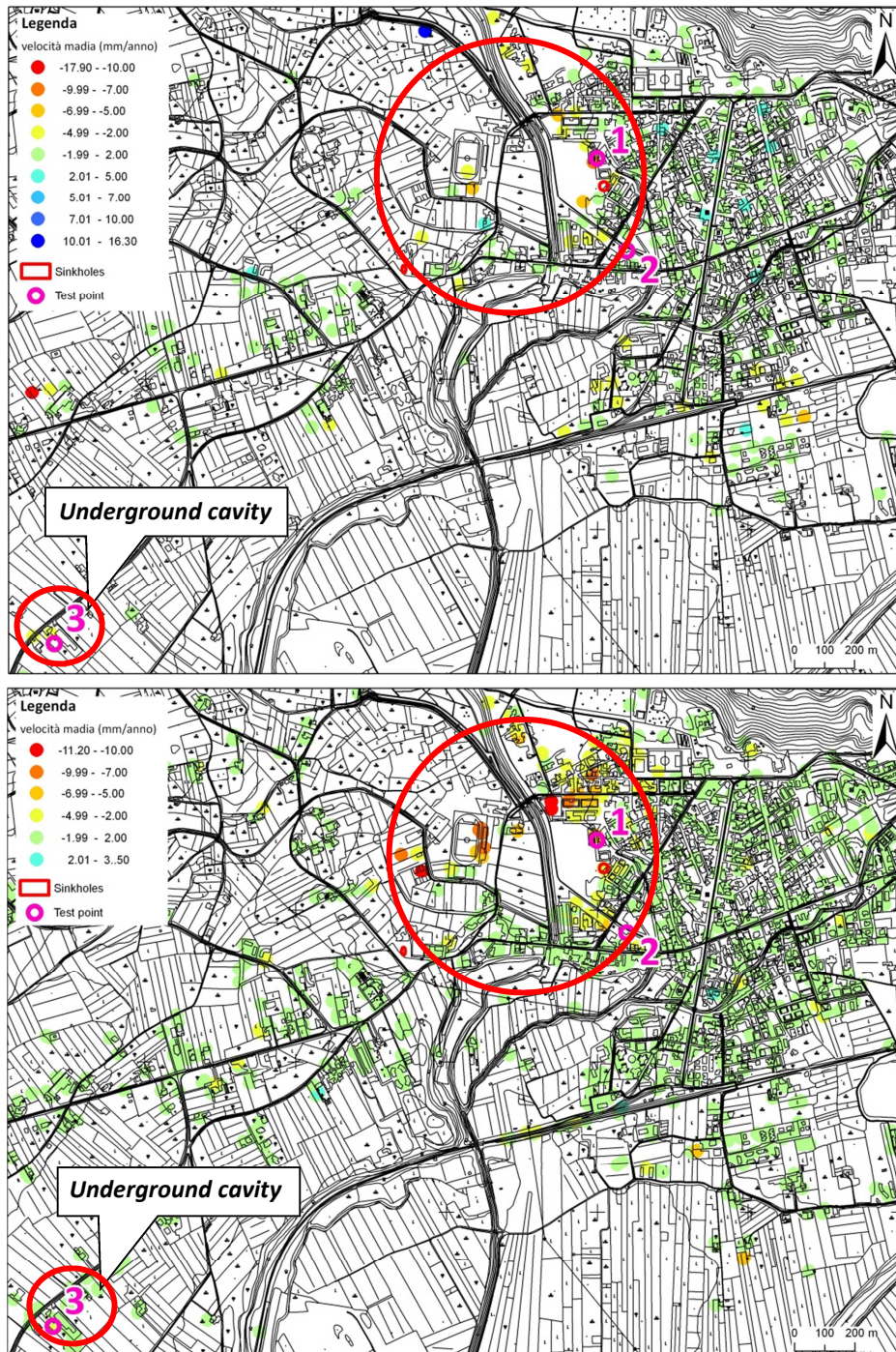
Figure 6.69: CPT processing results (above); PS DInSAR data (below)
