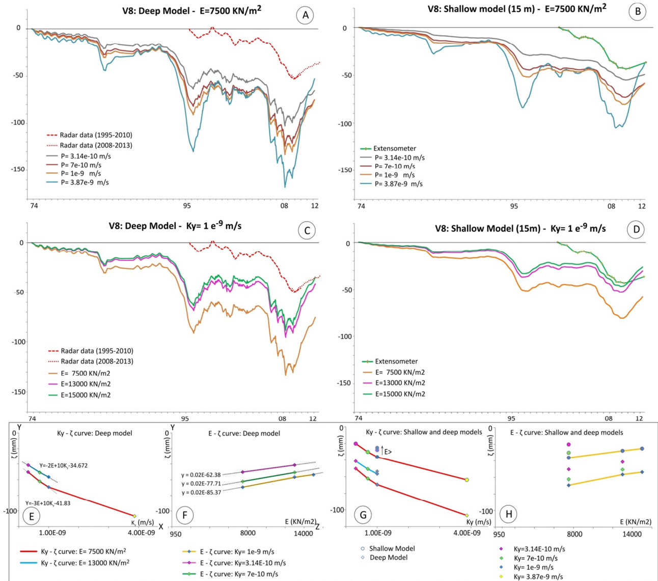
Figure 6.38. Analysis of the influence of E and K_y in the model
