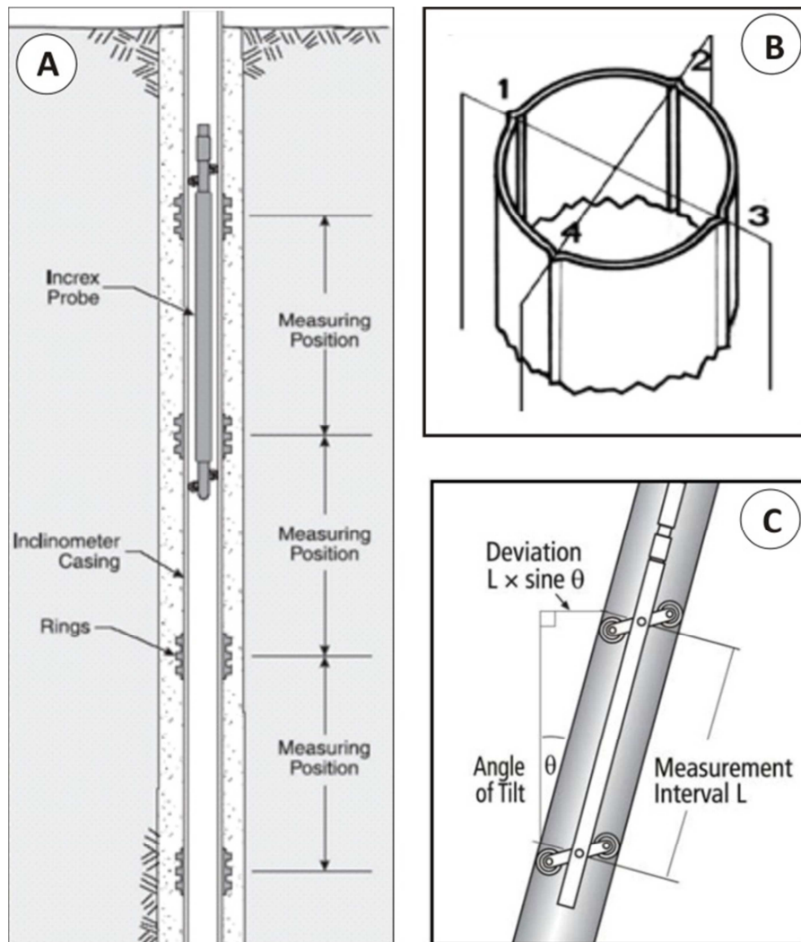
Figure 3.3: Inclinometer section (a); inclinometric grooves (b); angular measurements (c); ( http://www.howland.co.uk/ )
