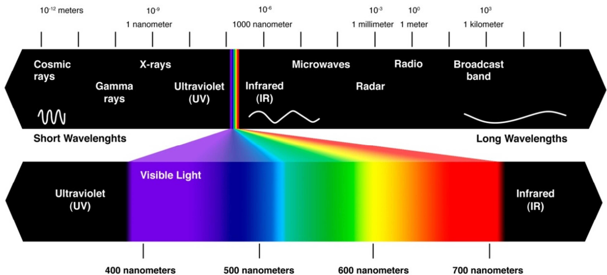
Figure 3.9: electromagnetic spectrum
