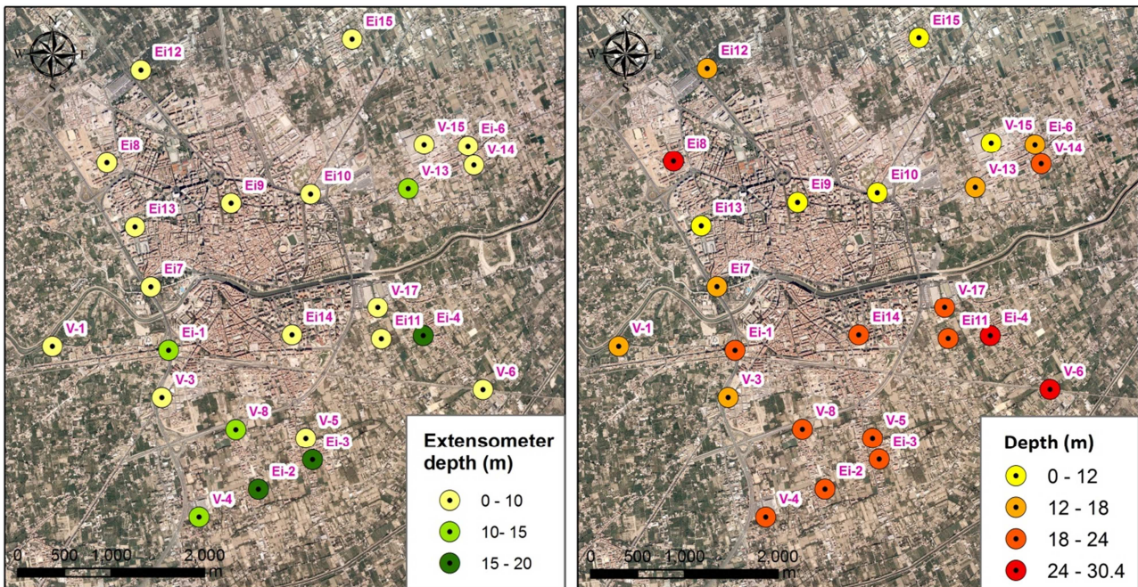
Figure 6.26: Extensometers depth (left); compressible material thickness (right)
